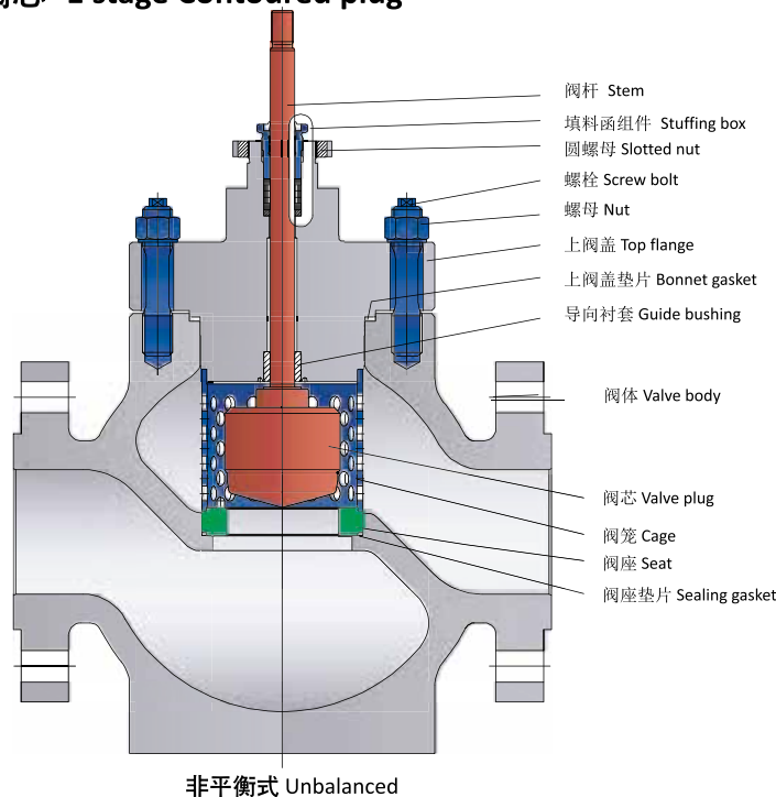
G150-C1 型结构图及部件图 (Sectional drawing of G150-C1) 一级抛物线型阀芯 1 stage Contoured plug
