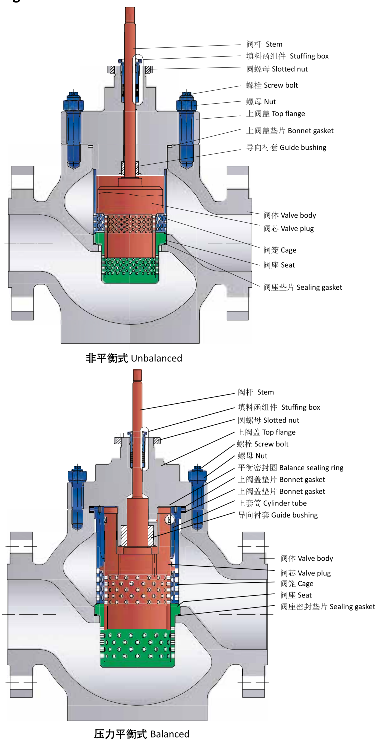
G150-H3 型结构图及部件图 (Sectional Drawing of G150-H3) 3 级多孔阀芯 3 stages Perforated trim
