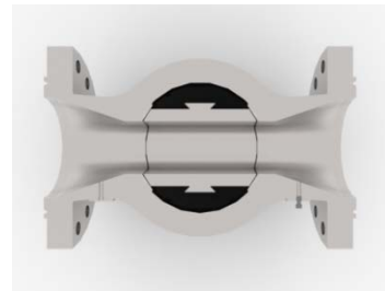
50~70% Reduced bore
