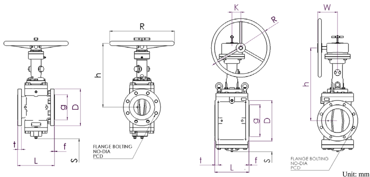
Figure No. 124 - Class 150 / Size 2" - 40" / Raised Face Flange
